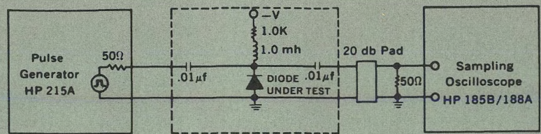
Test circuit for measurement of switching time ( T_s ).
