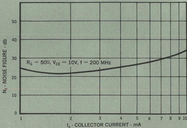
TYPICAL NOISE FIGURE vs COLLECTOR CURRENT
