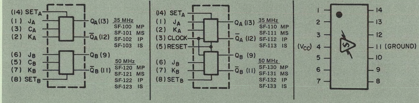
PIN BASING FOR SYLVANIA'S DUAL J-K FLIP-FLOPS
