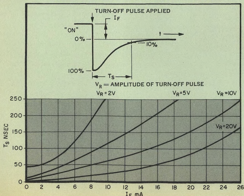
SWITCHING CHARACTERISTICS OF D-5720 "FAST" PIN DIODE
