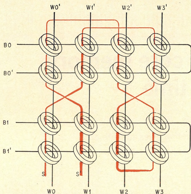
Sense winding run parallel to word windings, not bit windings as in some 2\frac{1}{2} -D memories. This diagram of a 4-by-4 array illustrates the winding layout and the "bow-tie" pattern. The inset shows how the bit line, lying between the sense and word lines, reduces coupling between them.
