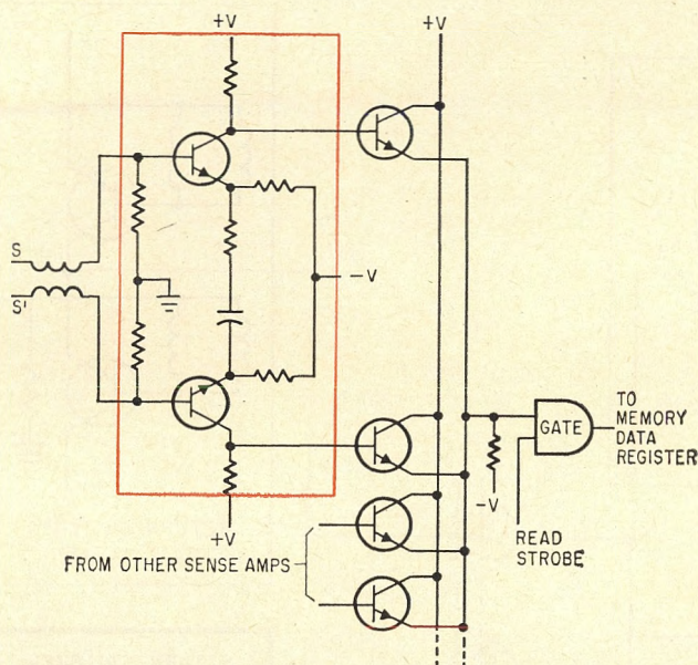
Sense amplifier connects eight sense windings to a single strobe gate through emitter-followers whose outputs share a common load. Differential preamplifiers (one of which is outlined in color) drive the emitter followers. This configuration keeps down the cost of sensing the many small sense sections in the memory.
