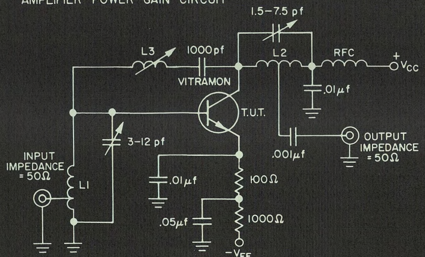
AMPLIFIER POWER GAIN CIRCUIT
