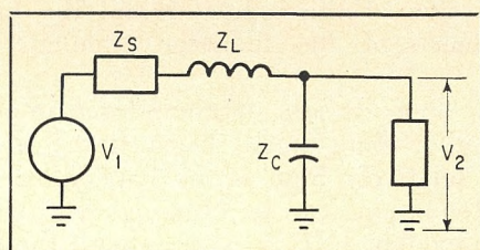
Simple L-section filter consisting of impedance Z_L and impedance Z_C is analyzed.
