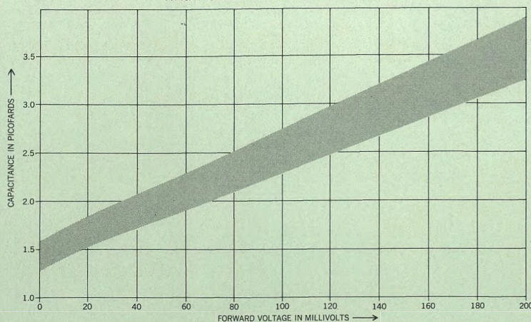
TYPICAL FORWARD BIAS CAPACITANCE DISTRIBUTION
