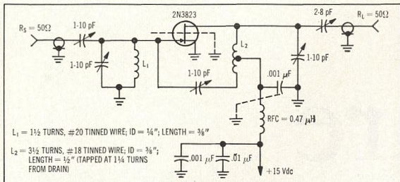
200 MHz Low-Noise Amplifier Circuit
